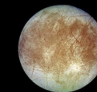
Europe
